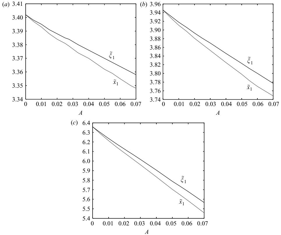
FIGURE 5. Plot of the neutral stability point for the Rankine body as a function of A for both \tilde{\zeta}_1 and \tilde{x}_1 for (a) \epsilon = 0.05 , (b) \epsilon = 0.1 and (c) \epsilon = 0.2 .
