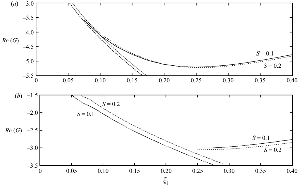
FIGURE 2. Plot of the real part of the growth rate G(\xi_1) as a function of downstream distance \xi_1 = 2\epsilon^2 \xi_R / U_0^2 , calculated by the leading edge receptivity analysis and local PSE theory, for S = 0.1 and S = 0.2 for the cases (a) \epsilon = 0.05 and (b) \epsilon = 0.1 .
